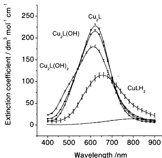
Fig. 5 Visible spectra of the species CuLH_2 , Cu_2L , Cu_2L(OH) , and Cu_2L(OH)_2 calculated from the spectrophotometric titration data.
