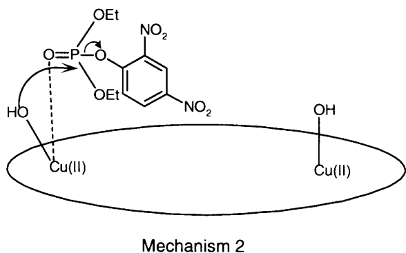
Fig. 7 Diagram showing the mechanism of \text{Cu}_2\text{PEA} promoted hydrolysis of DNPDEP.
