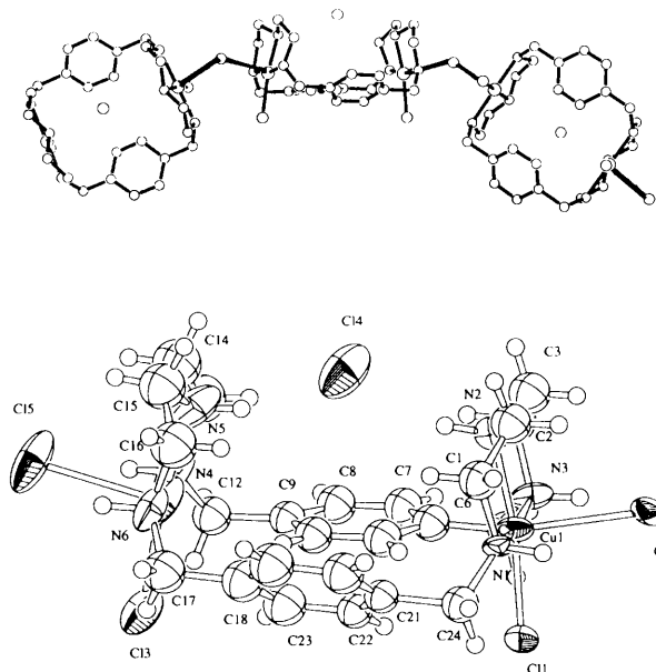
Fig. 2 An ORTEP 19 diagram of [Cu 2 (PEA)Cl 3 ] + Cl - ·2.6MeCN·2.9H 2 O showing the atom labeling scheme and ball-and-stick diagram showing chloro-bridging. Solvent molecules not shown. Thermal ellipsoids are at 50% probability.
